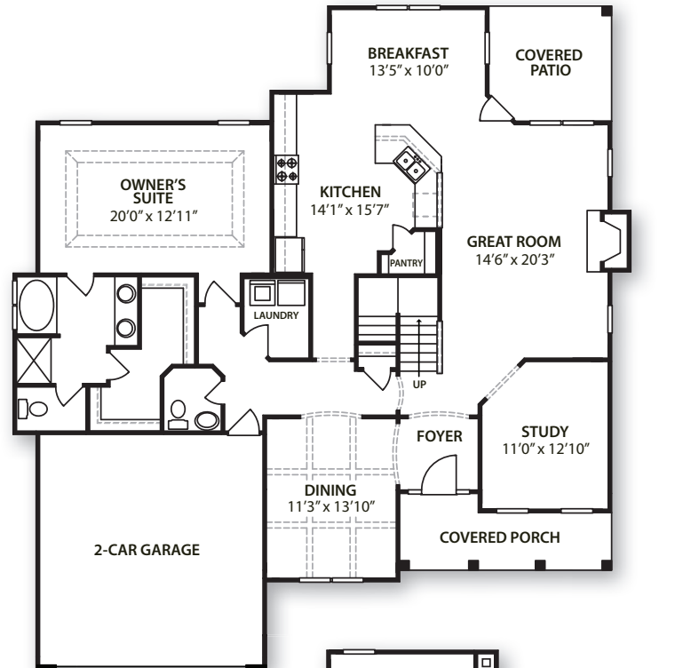
FIRST FLOOR
